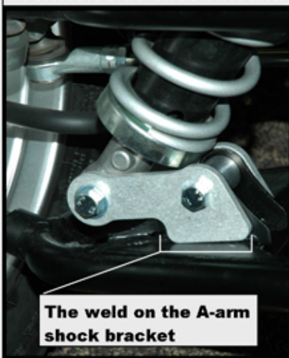
Front left side shock mount.
